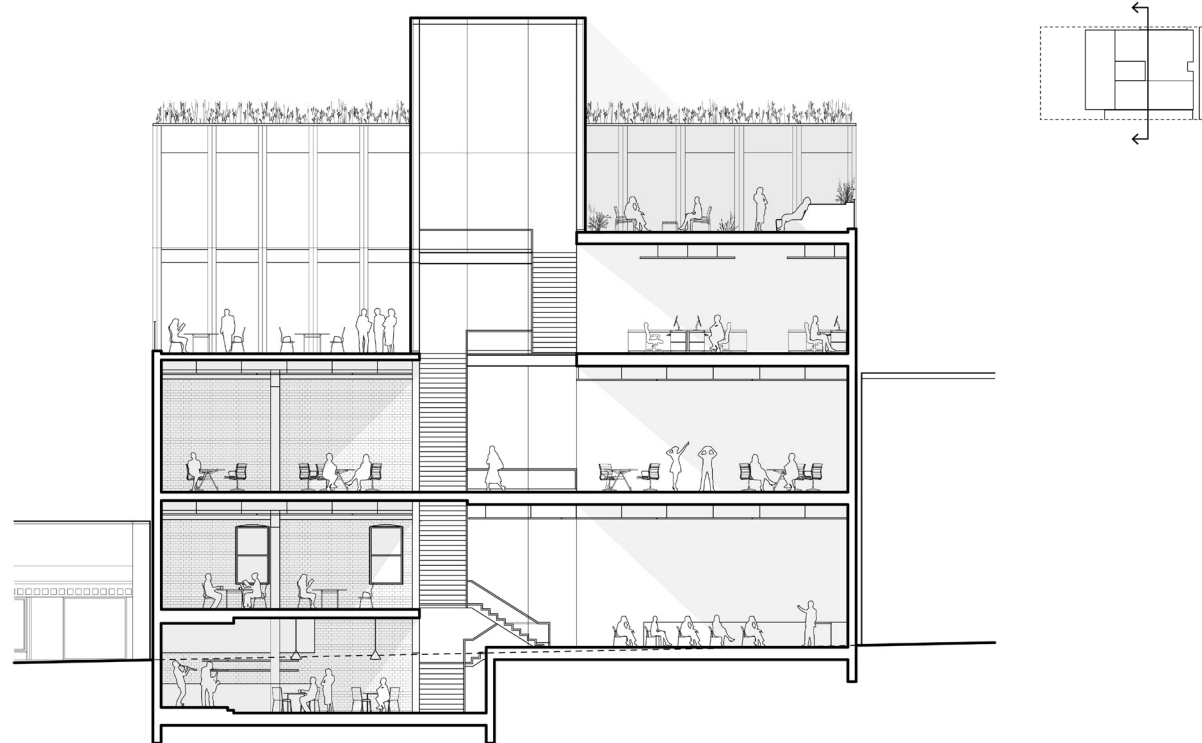
Section // Looking, Northwest
