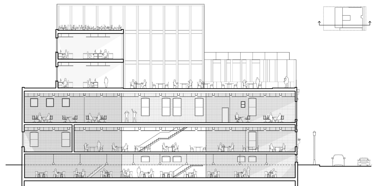
Section // Longitudinal, Looking Northeast
